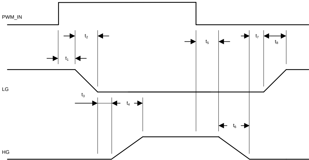
Figure 2. Timing Diagram
